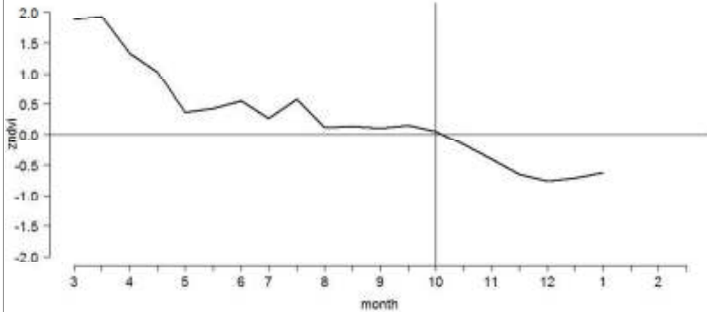
Figure 1. ZNDVI in North Horr from March 2010 to February 2011
