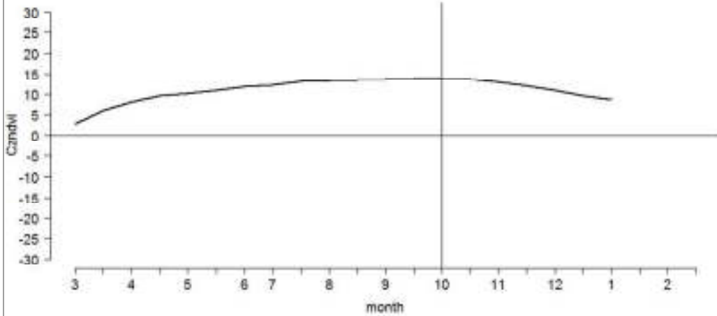
Figure 2. Czndvi in North Horr from March 2010 to February 2011
