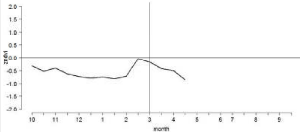
Figure 1. ZNDVI in Maikona from October 2010 to September 2011
